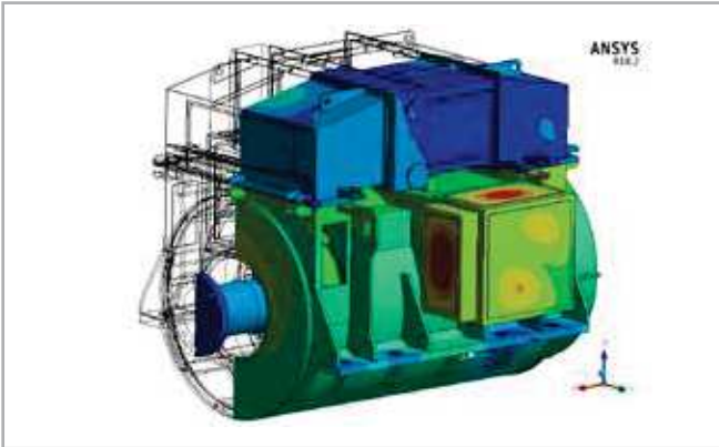
Max power generator in a marine application and simulation of its alternator
