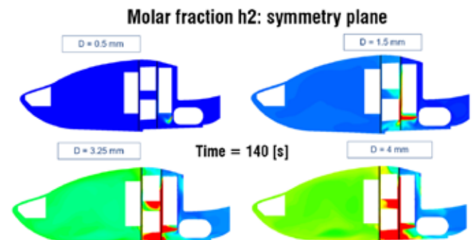
Fig.6. Hydrogen mole fraction for different leak sizes (forced ventilation).
