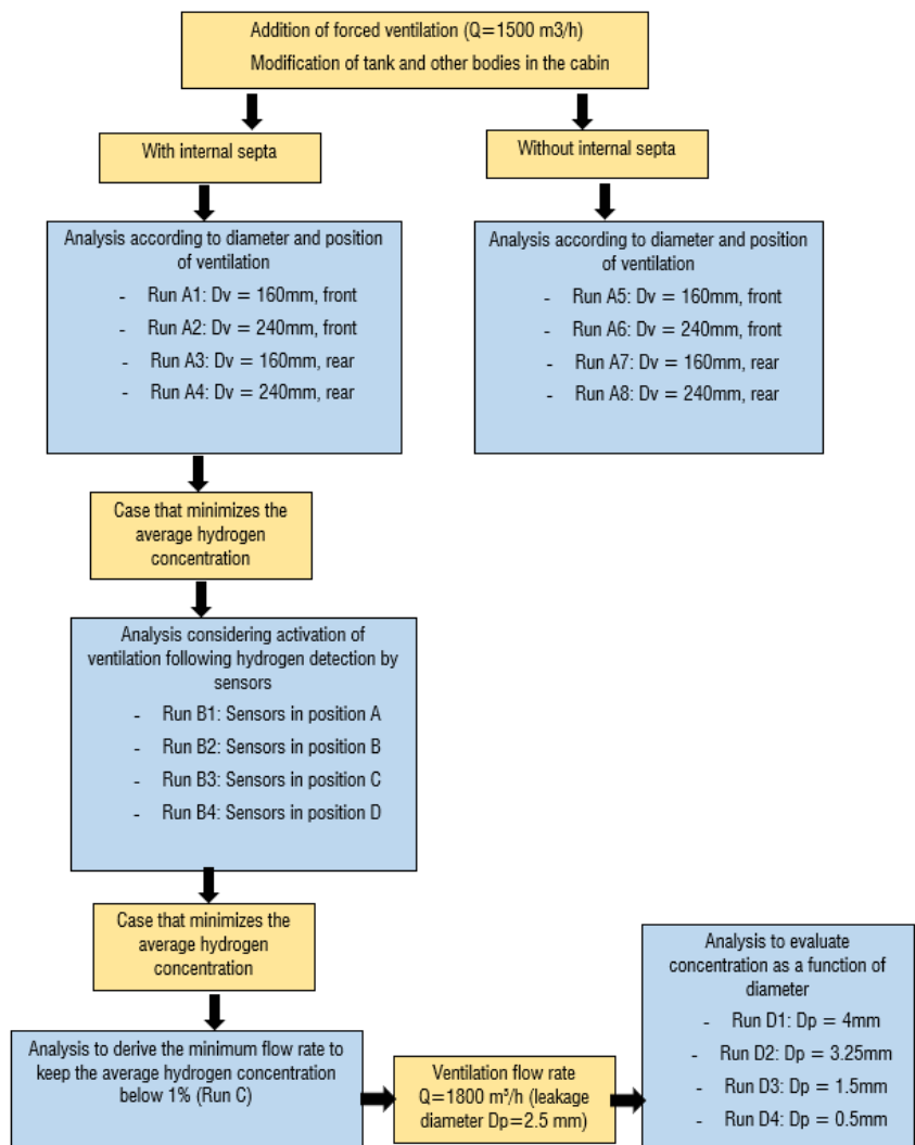
Fig.7. Logical scheme followed to carry out the simulations.
