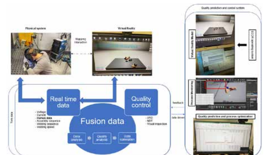
Fig.4. Digital Shadow model to predict and control manual welding quality.
