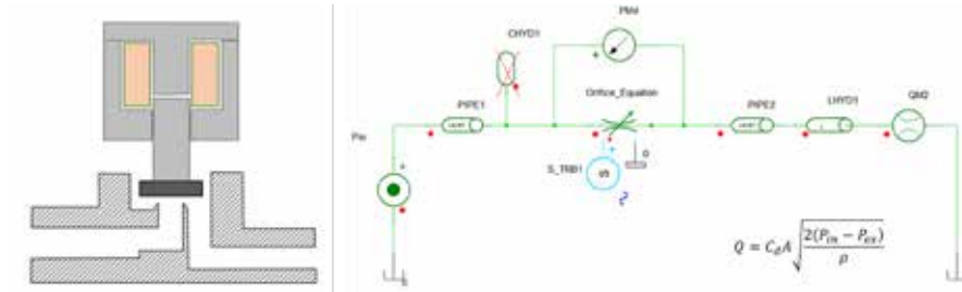
Fig. 6. System modelling of a fluid valve.
