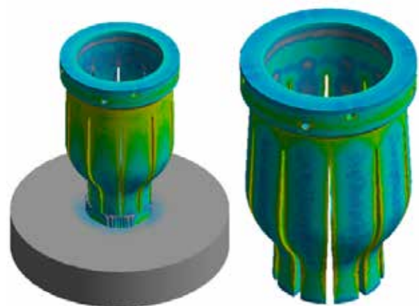
Fig. 9. Stress on the part in the as-built condition after process simulation Left) job anchored to the platform. Right) after detachment of the part from the platform and the removal of supports.
