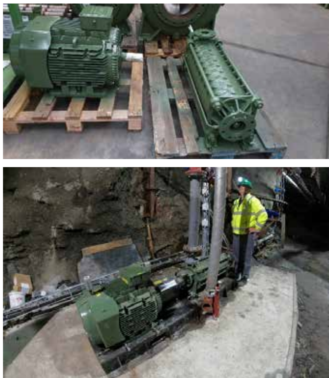
Fig. 2. SAER multistage turbine model E-TMZ-4P-50-80. Top: during manufacture; bottom: after installation.
