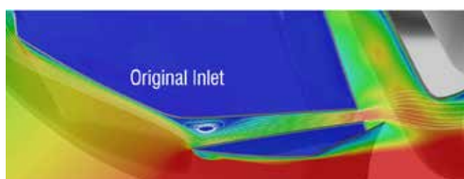
Most ducts inlets have significant recirculation. But if the designer understands the flow paths over the fascia while creating the design concept shape the result can be a duct with twice the flow potential.
