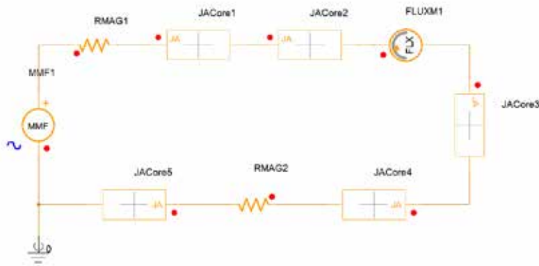
Fig. 2. Equivalent magnetic circuit of a solenoid valve.
